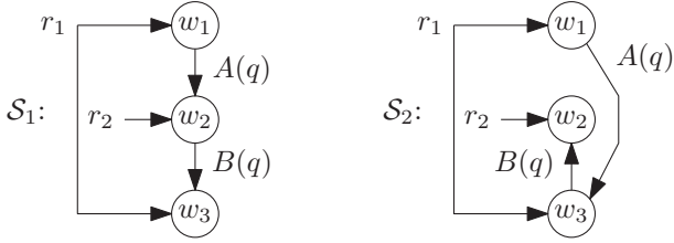
Fig. 1. Systems \mathcal{S}_1 and \mathcal{S}_2
