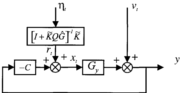
Figure 6.4. Simplified closed loop
