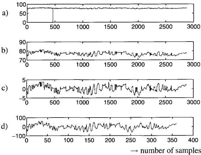
Figure 6.5. Measured internal reflux-to-feed ratio (a), after outlier correction (b), trend removal (c) and decimation and scaling (d)
