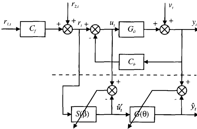
Figure 2.3. Schematic drawing of the Two-Step method (TS), with the upper part denoting the real system, and the lower part denoting the models involved
