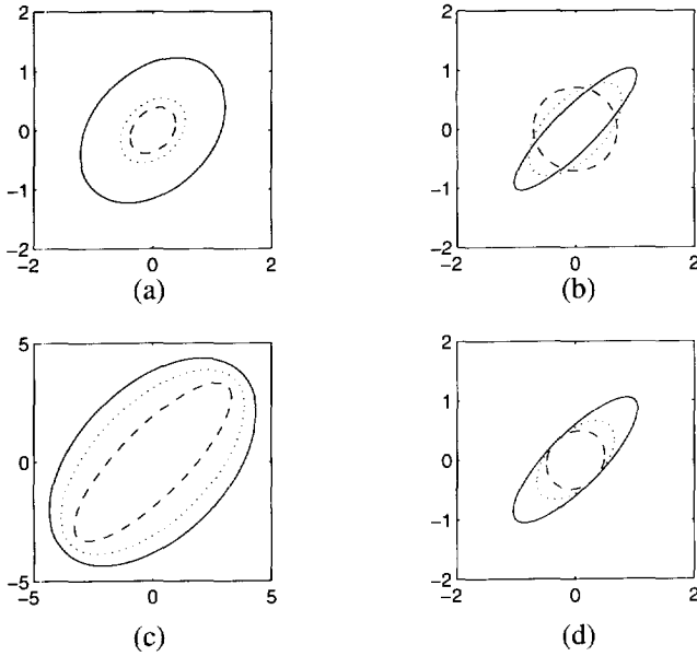
Figure 5.2. Iso-Vs for different experiments
