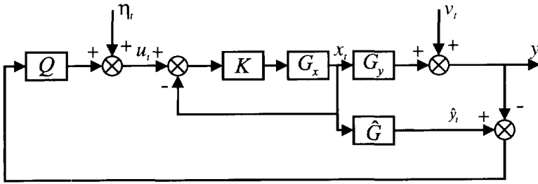
Figure 6.3. Control configuration
