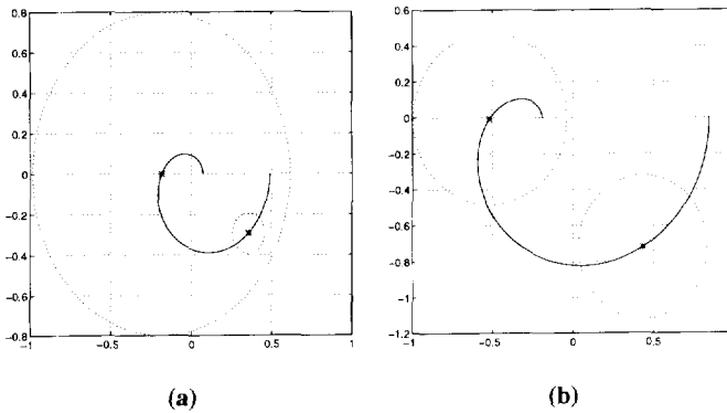
Figure 5.1. Nyquist diagram (solid) and uncertainty intervals (dotted) of a loop transfer function \hat{G}C for different uncertainty distributions
