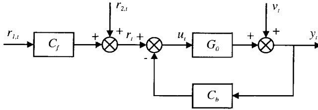
Figure 2.2. Closed-loop control configuration
