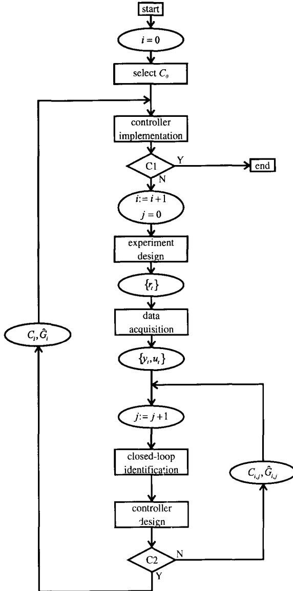
Figure 4.1. Iterative scheme of identification and control design
