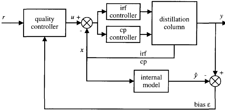
Figure 6.2. Control configuration of the distillation column, shown in Figure 6.1
